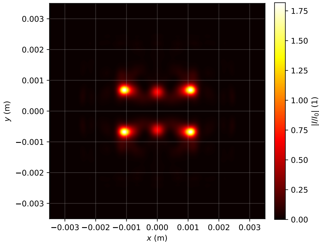
Intensity profile I(x, y, z = 2.070)/I_0 , P_{in}=7.0P_{cr} , artificial time
